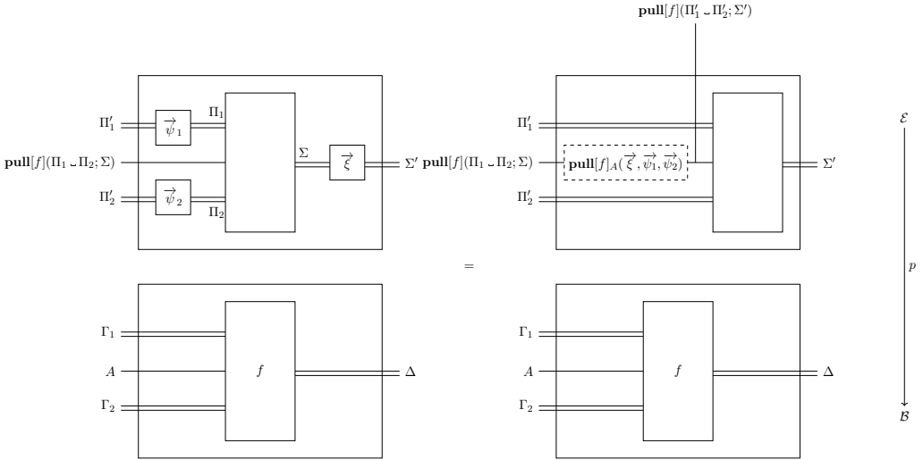
Fig. 1. Polymap \mathbf{pull}[f](\Pi_1 \dashv \Pi_2; \Sigma) \rightarrow \mathbf{pull}[f](\Pi'_1 \dashv \Pi'_2; \Sigma')
